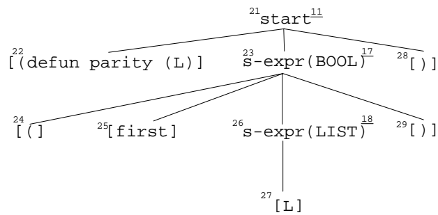
Figure 2: The derivation tree of the second program.
