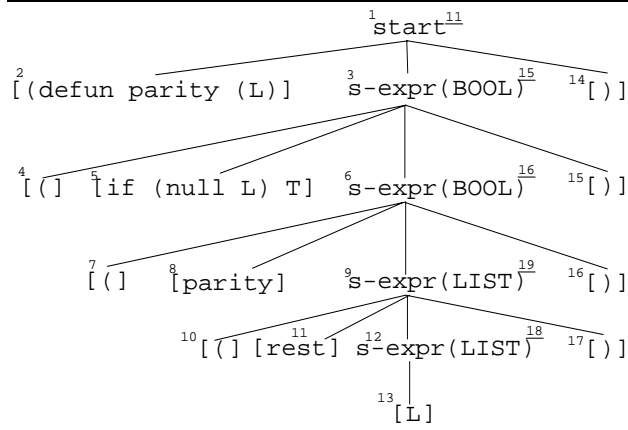
Figure 1: The derivation tree of the first program.
